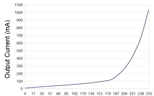
Logarithmic dimming
